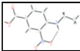
Fig. 1. The molecular structure of the title compound, showing 50% probability displacement ellipsoids and the atom numbering scheme. The dashed line indicates an intramolecular hydrogen bond.
