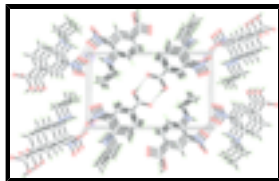
Fig. 2. The crystal packing of the title compound, viewed along the a axis. Hydrogen bonds and the short O...O contacts are shown as dashed lines.
